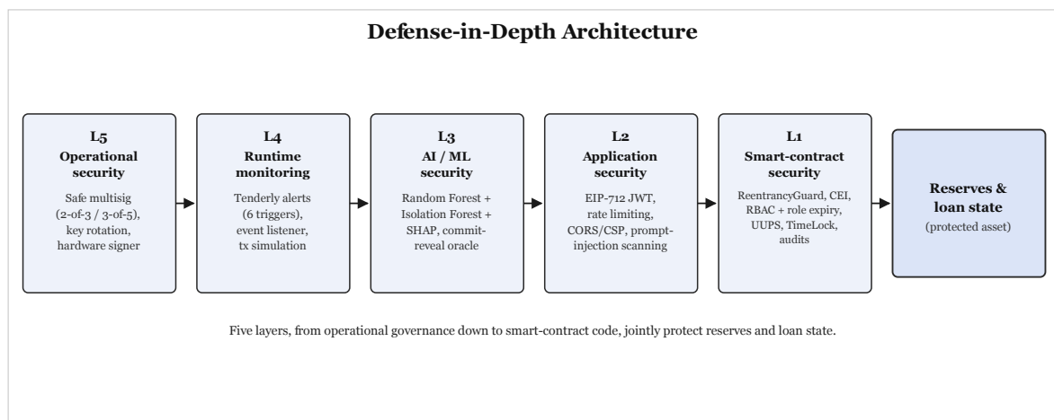
Figure 4.42: Defense-in-depth architecture.
